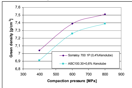
Figure 8: Compressibility curve of Somaloy 700 and ABC 100.30 (400MPa=28,8tsi; 600MPa=43,2tsi; 800MPa=57,6tsi)
