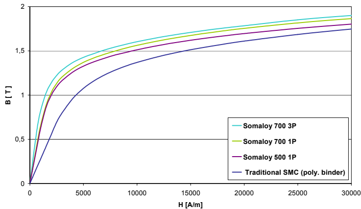
Figure 7: B-H curve
