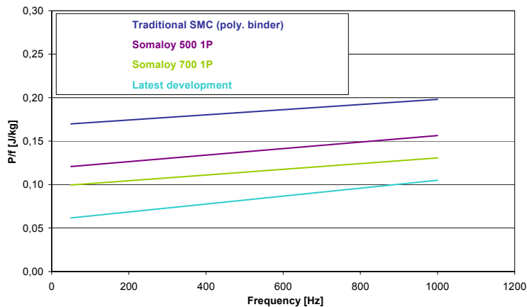
Figure 6: Losses/cycle (Core loss /frequency) plotted as function of frequency
