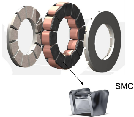
Figure 3: Axial flux motor designed and build by Oxford University
