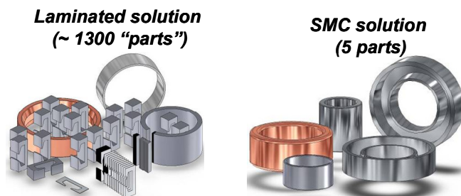
Figure 5: Parts required for laminated and SMC solution
