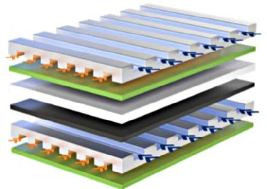
Principle setup of Solid Oxide Cell
